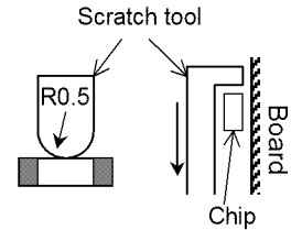
Cross Section
